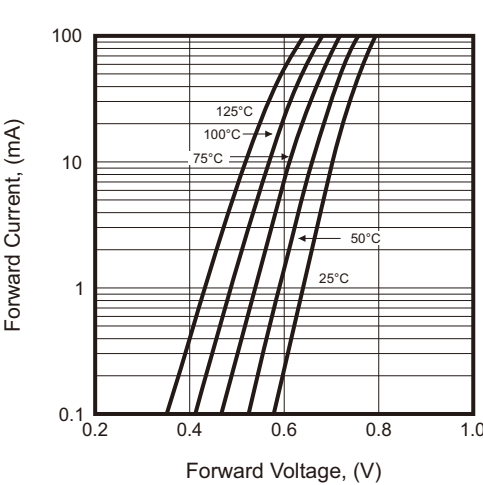
Fig.5 - Forward Characteristic
