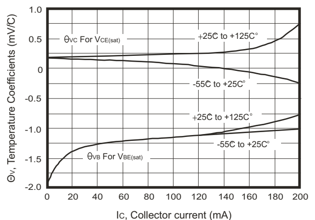
Fig. 12- Temperature coefficients
