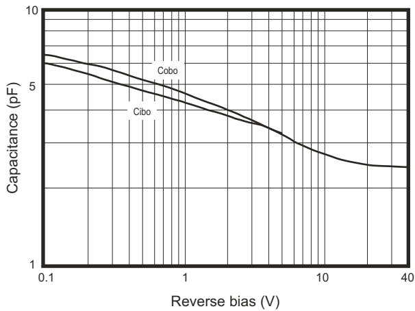
Fig.1 Capacitance
