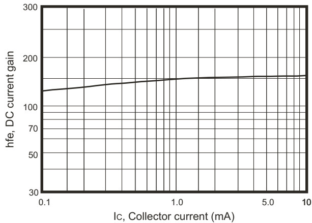
Fig.7 Current gain
