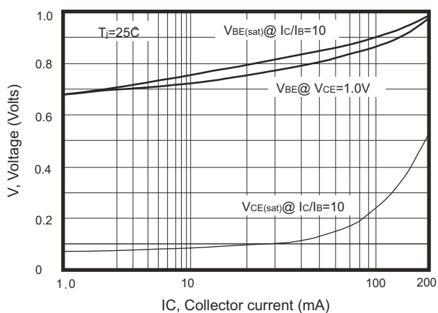
Fig. 11- "ON" voltages
