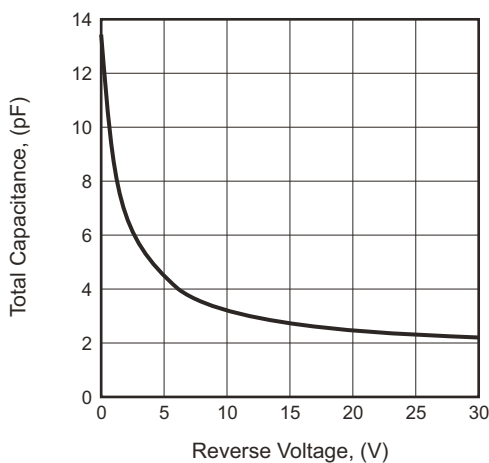
Fig.3 - Total Capacitance
