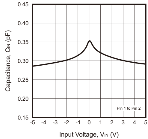
Fig.2 - Typical Variation of C_{IN} VS. V_{IN}
