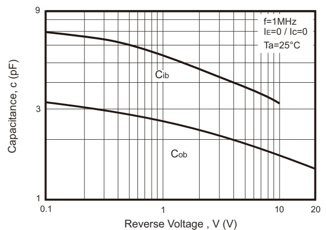
Fig. 6 - C_{ob}/C_{ib} - V_{CB}/V_{EB}
