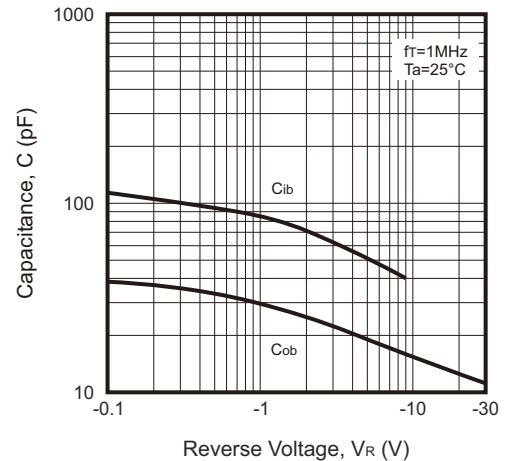
Fig.6 - C_{ob}/C_{ib} \sim V_{CB}/V_{EB}
