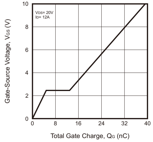
Fig.8 - Gate-Charge Characteristics
