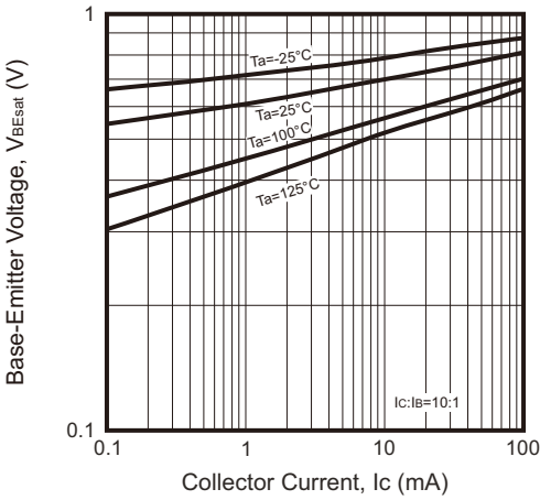
Fig.4 - Base-Emitter Saturation Voltage
