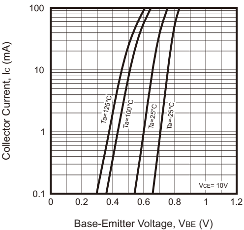
Fig.5 - Base-Emitter on Voltage
