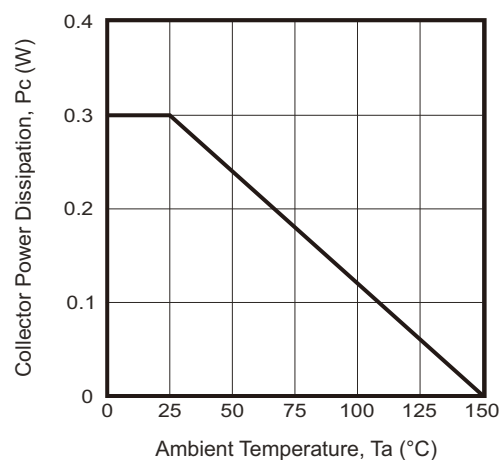
Fig.8 - P_C - T_A
