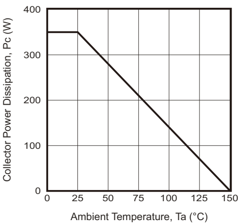
Fig.7 - P_C - T_a
