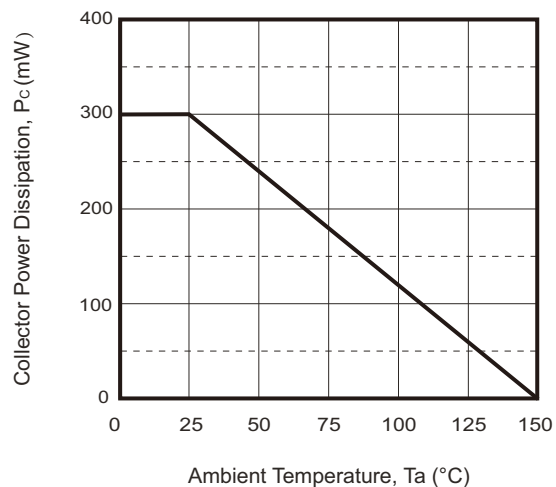
Fig.8 - P_C - T_a
