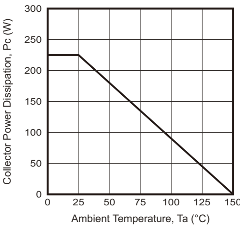
Fig.7 - P_C — T_a
