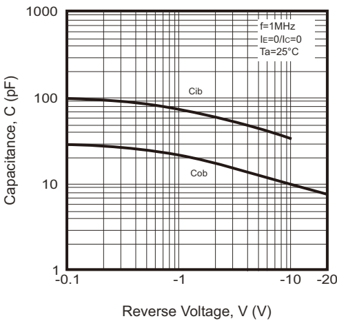
Fig.5 - C_{ob}/C_{ib} — V_{CB}/V_{EB}
