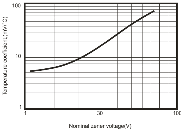
Fig.3 Temperature coefficients
