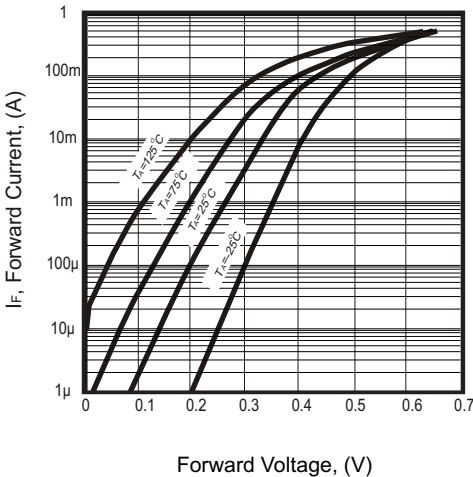
Fig.1 - Forward Characteristics
