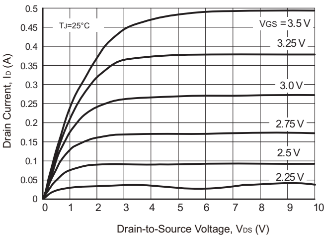
Fig.2 - On-Region Characteristics
