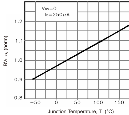
Fig.9 - BV_{DS} vs Junction Temperature
