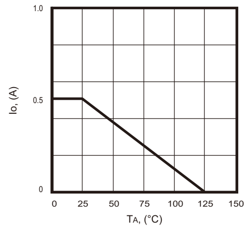
Fig.4 - Derating Curve
