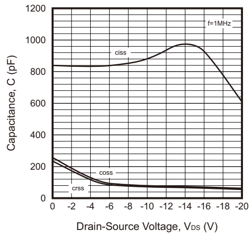
Fig.6 - Capacitance
