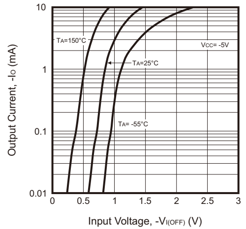
Fig.6 - Output Current vs Input Voltage
