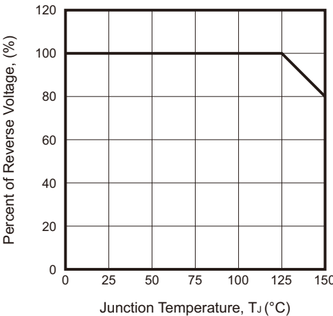
Fig.5 - Operating Temperature Derating Curve
