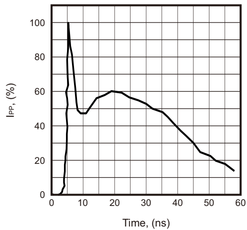
Fig.7 - ESD Pulse Waveform IEC 61000-4-2
