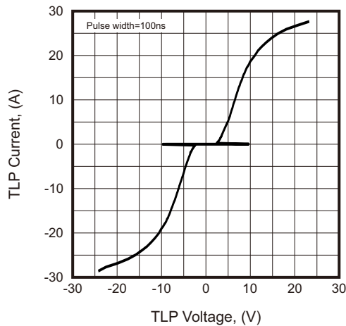
Fig.5 - TLP Curve
