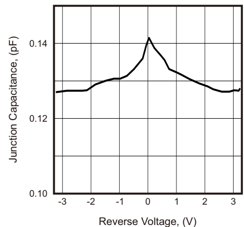
Fig.4 - Junction Capacitance Curve
