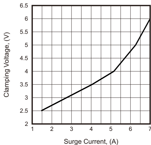
Fig.3 - 8/20μs Surge Curve
