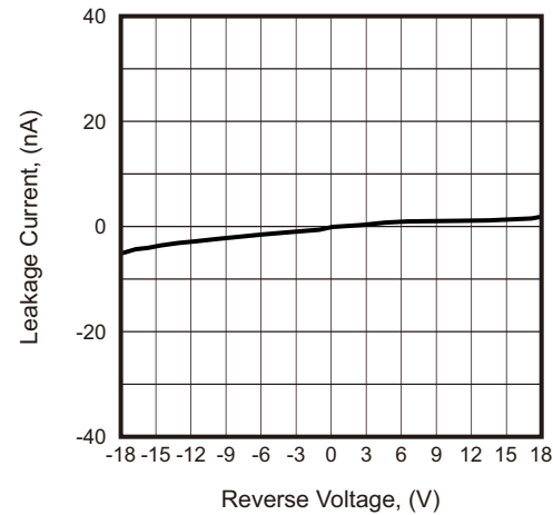
Fig.2 - Leakage Current Curve
