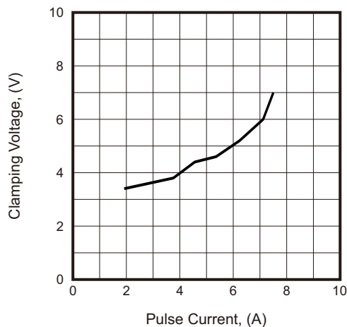
Fig.3 - 8/20μs Surge Current Curve
