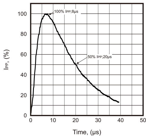
Fig.5 - 8/20μs Pulse Waveform IEC 61000-4-5
