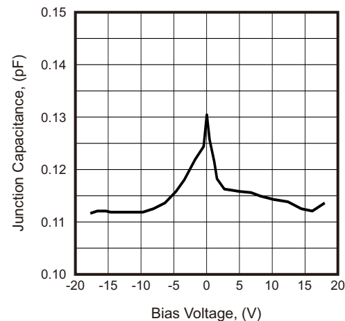
Fig.4 - Junction Capacitance Curve
