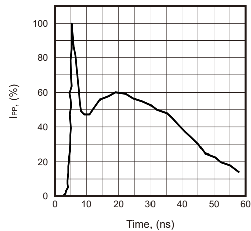
Fig.6 - ESD Pulse Waveform IEC 61000-4-2
