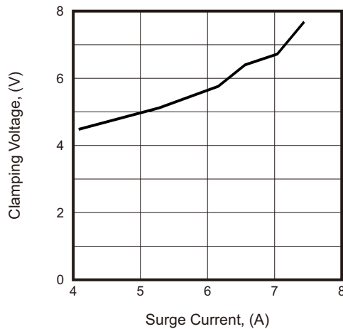
Fig.3 - 8/20µs Surge Curve
