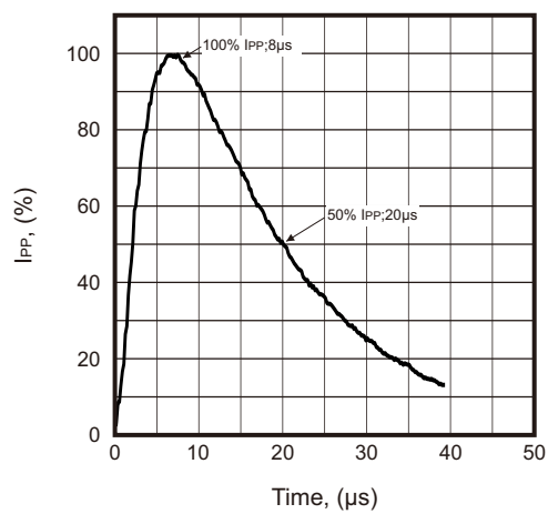
Fig.6 - 8/20µs Pulse Waveform IEC 61000-4-5
