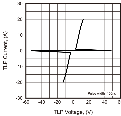
Fig.5 - TLP Curve
