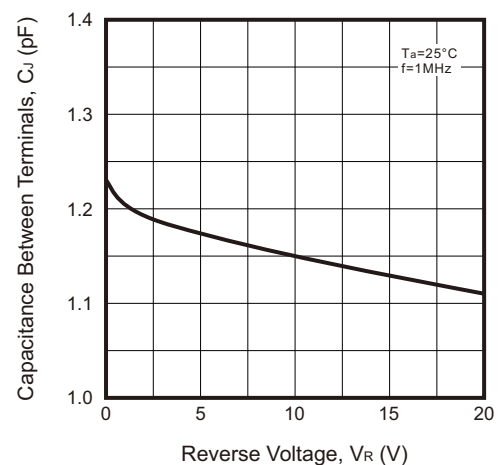
Fig.4 - Capacitance Characteristics
