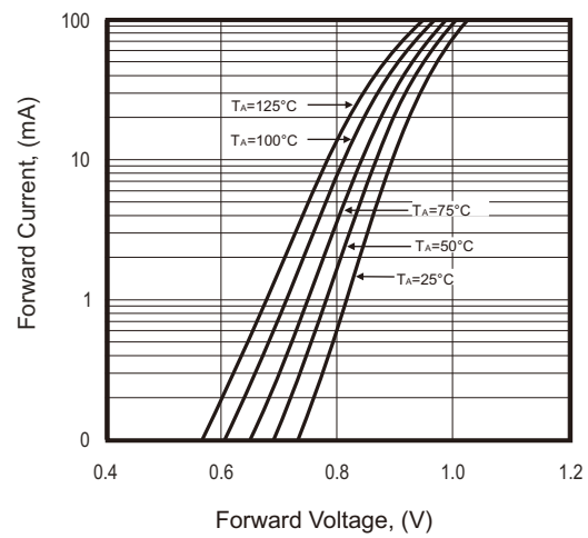
Fig.2 - Forward Characteristics
