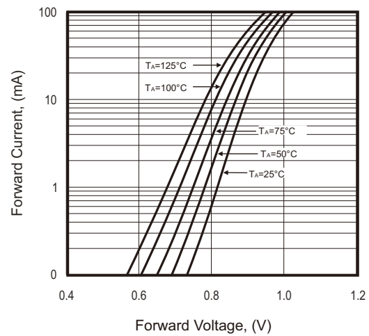
Fig.2 - Forward Characteristics
